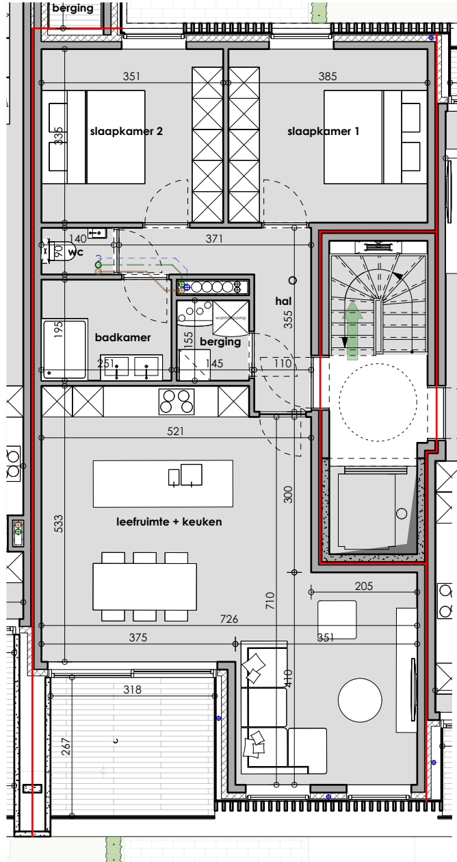
GRONDPLAN BASIS 0 1 2m
